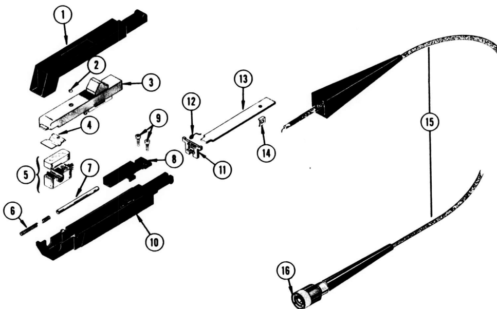
P6021 PROBE
