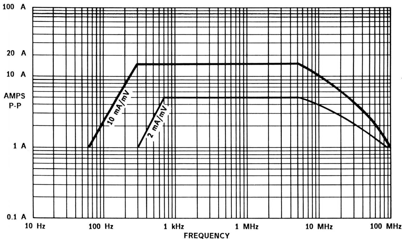
Fig. 1-2. P6021/Termination Input Current vs Frequency Derating.
